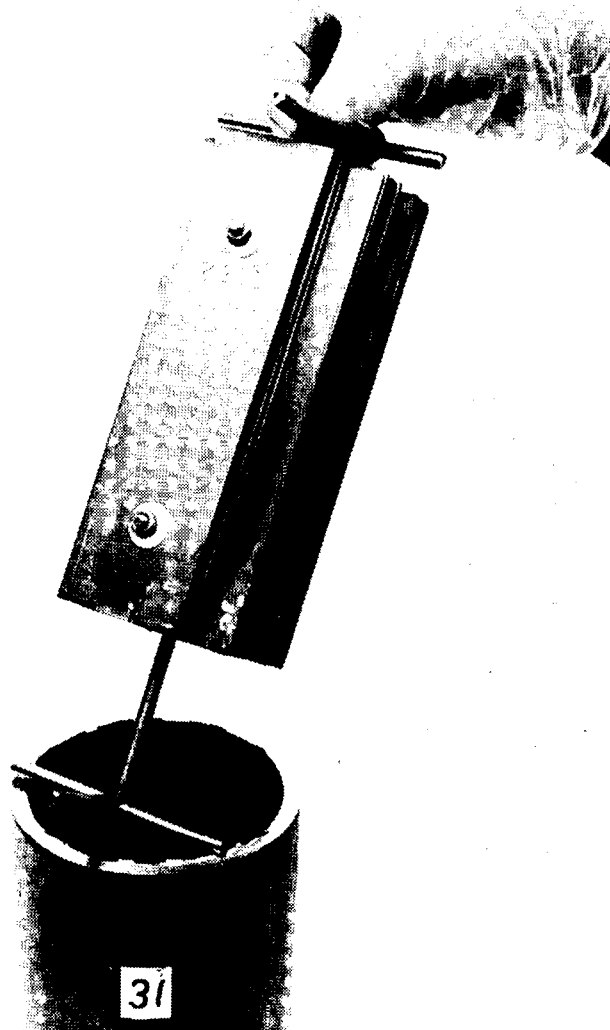
Figure 6-7. Post-test appearance of steel specimens, vapor-phase exposure, 24-month brine/ \text{CO}_2 tests. No significant corrosion reaction is evident except where brine has contacted the bottoms of the specimens.
